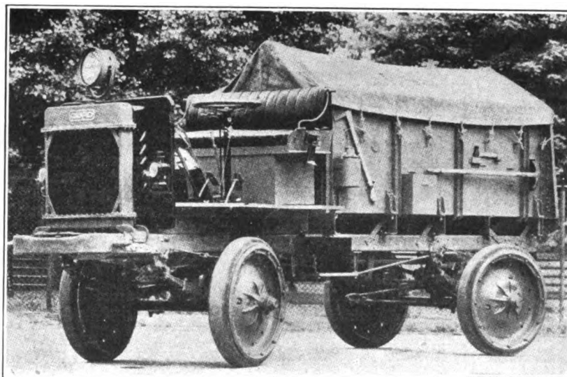
Perspective View Standard Ammunition Body
